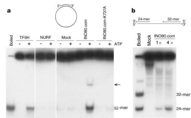
Figure 3 INO80 complex has 3' to 5' specific helicase activity. a , Native PAGE (10%) showing the displacement of a 32 P-labelled 52-mer annealed to circular single-stranded \Phi X174 DNA on incubation with the indicated reagents. (INO80.com also produces a weak band (arrow), which may be a metastable intermediate.) b , Native PAGE (10%) showing the displacement of the 32 P-labelled 24-mer or 32-mer. 1× and 4× refer to concentrations of INO80 complex. All reactions contained ATP. Structures of substrates are shown on top and the 32 P-label is indicated by an asterisk.
