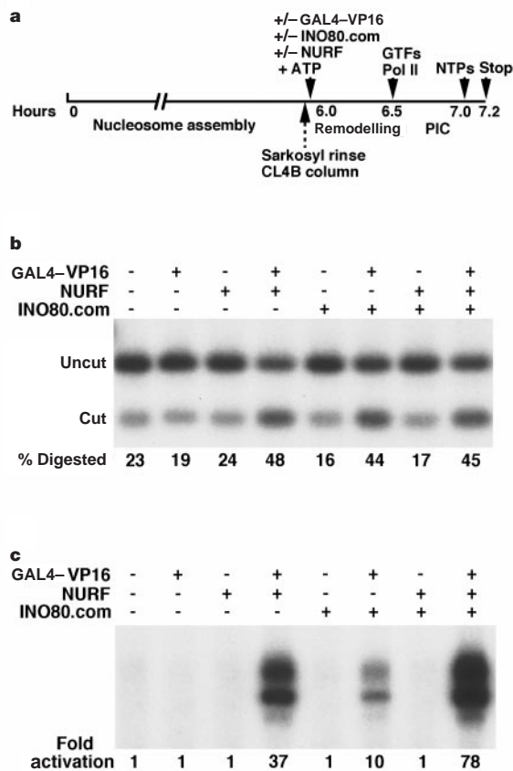
Figure 4 INO80 complex remodels and promotes transcription from a chromatin template. a , Protocol. b , Southern blots showing that both NURF and the INO80 complex enhance digestion of a Pst I- Cla I fragment (uncut) by Bam HI (cut). c , Transcription analysis of remodelled chromatin templates. Primer extension of transcripts from the E4 promoter (+99 to +72 primer). ATP was present in all reactions and was needed for the remodelling step.
